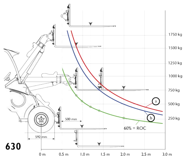
Lastdiagram 630/635/640
