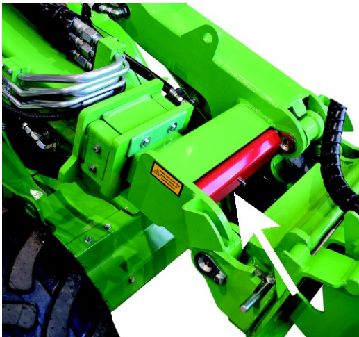
Cylindersikring, monteret
